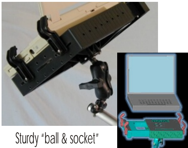
Wide adjustment for boom arm angle, and the Ball & Socket joints of the LCD or Laptop mounts keep them level.
